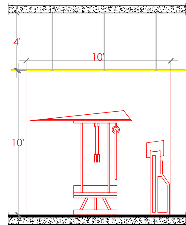
SECTION - C3
