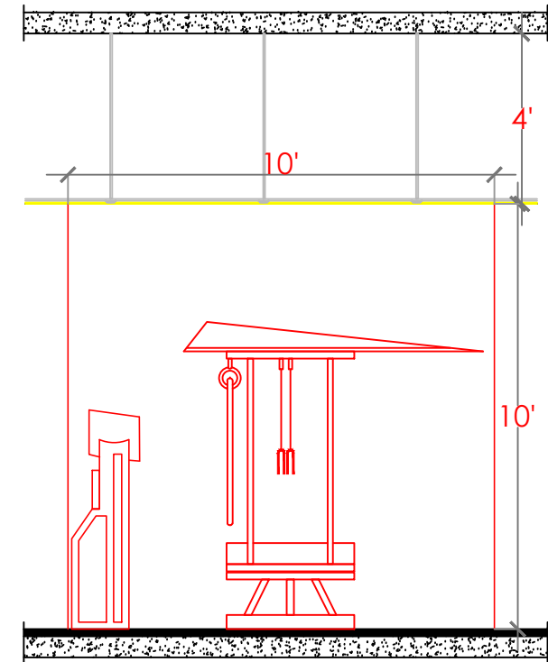
SECTION - C2
