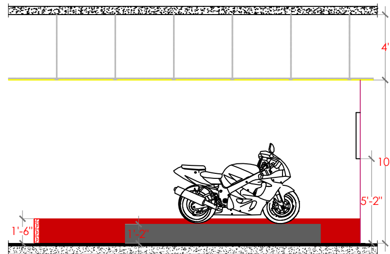
SECTION - I3
